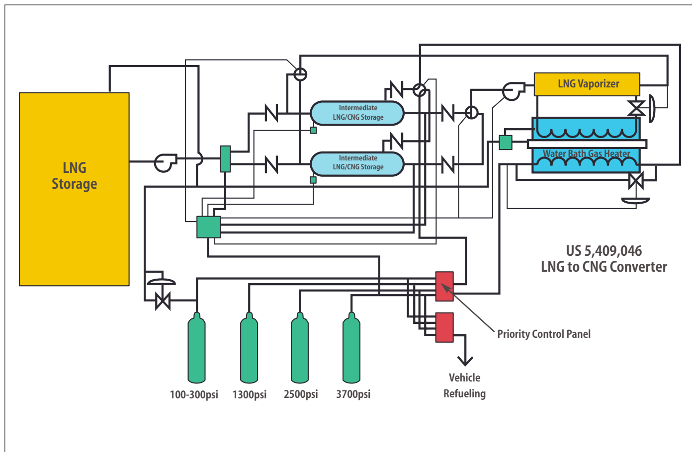
Figure 1: LNG TO CNG converter. Courtesy of Wolf Koch. US patent number US 5,409,046.
