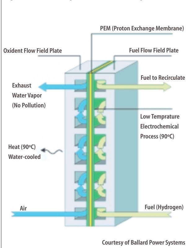
Figure 4: Proton exchange membrane fuel cell diagram.
