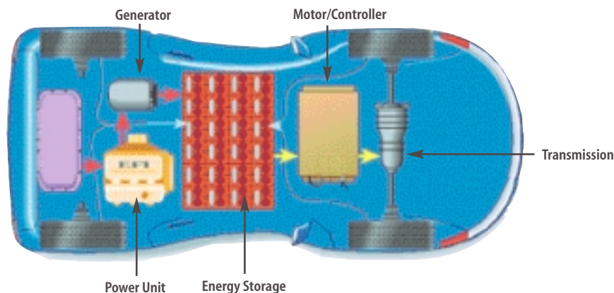
Figure 3: A hybrid electric vehicle with a series or "range extender" configuration.
