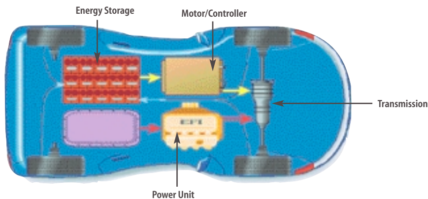
Figure 2: A hybrid electric vehicle with a parallel or "power assist" configuration.
